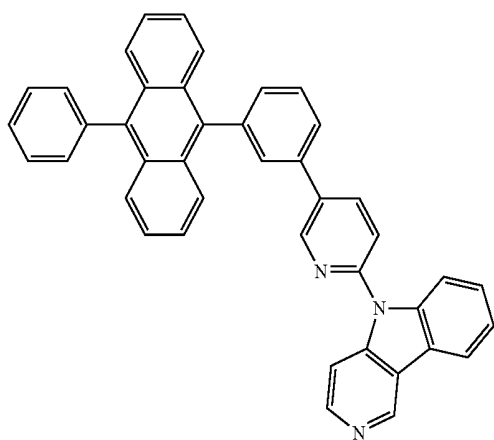
[Chemical Formula 82]
