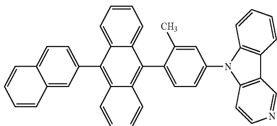
(Compound 10)
