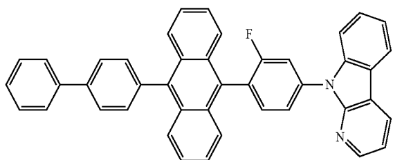
(Compound 8)
