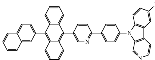
[Chemical Formula 81]
