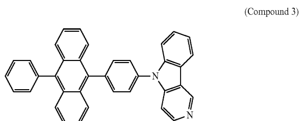
[Chemical Formula 3]
