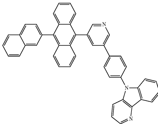
[Chemical Formula 85]
