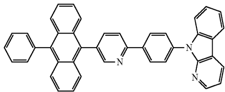
[Chemical Formula 80]
