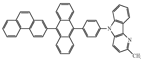
(Compound 13)
