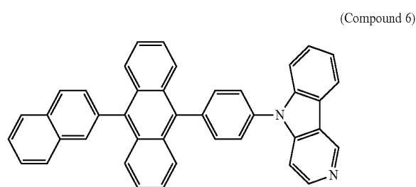
[Chemical Formula 6]
