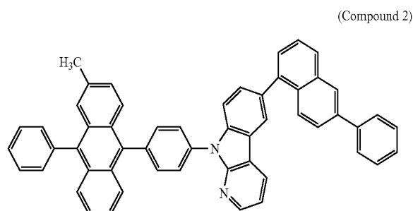
[Chemical Formula 2]
