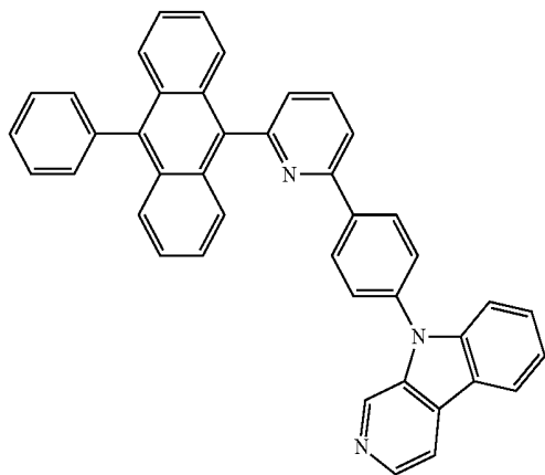
[Chemical Formula 84]
