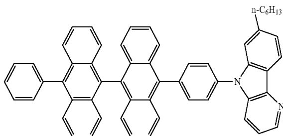
(Compound 14)
