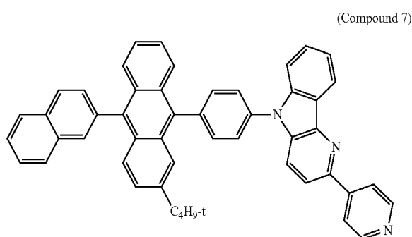
[Chemical Formula 7]
