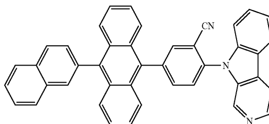
(Compound 11)
