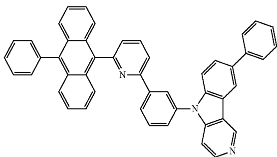
(Compound 84)
