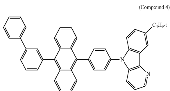
[Chemical Formula 4]
