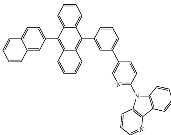
[Chemical Formula 83]
