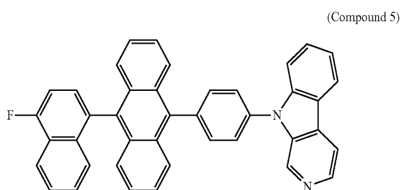
[Chemical Formula 5]
