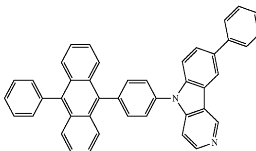
(Compound 15)
