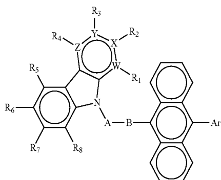
[Chemical Formula 1]
